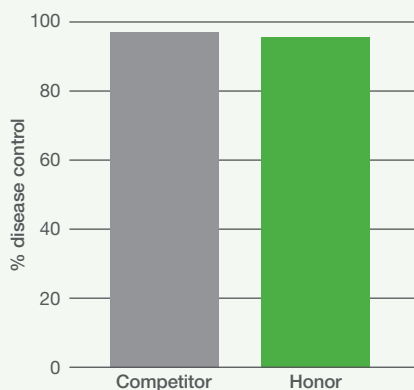
Anthracnose control plus Intrinsic Plant Health Benefits 1
