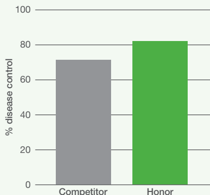
Summer patch control plus Intrinsic Plant Health Benefits 1
